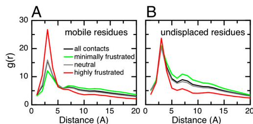
Fig. 2. Local frustration and residue displacement. The pair-distribution functions between the C\alpha of the residues classified by displacement and the center of mass of the contacts in different frustration classes was computed. The distributions for all contacts (black), minimally frustrated (green), neutral (gray), or highly frustrated contacts (red), are shown for the mobile (A) or undisplaced (B) residues.
